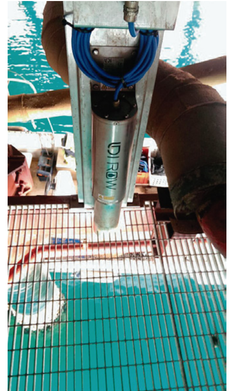
Oil Terminal, Italy
